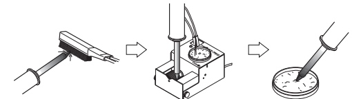
(1) Remove oxide with a brush. (2) Clean with the HAKKO FT-700 again. (3) Tin with the HAKKO FS-100 again.
